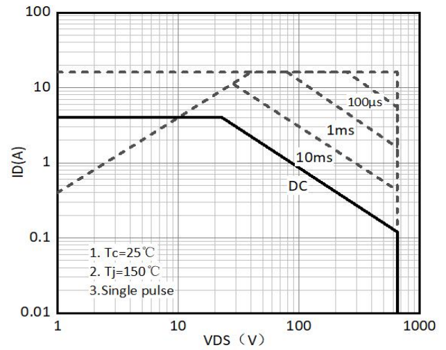
Figure 10. Safe Operating Area (TO-251 TO-252)
